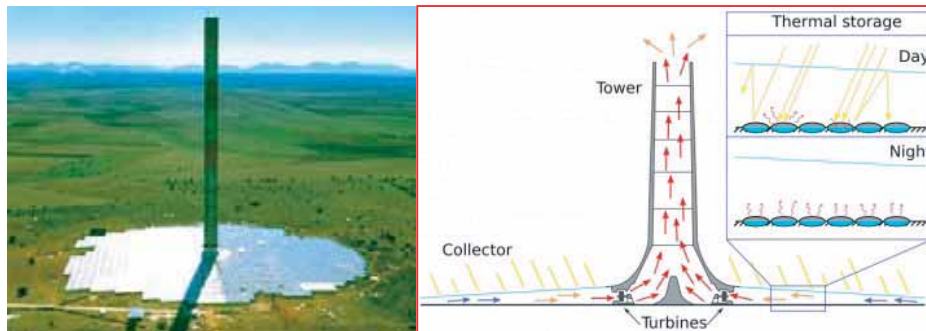
Solar Chimney
