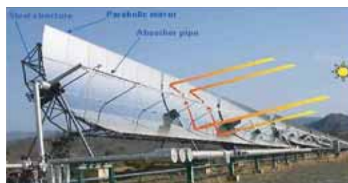
Parabolic trough
