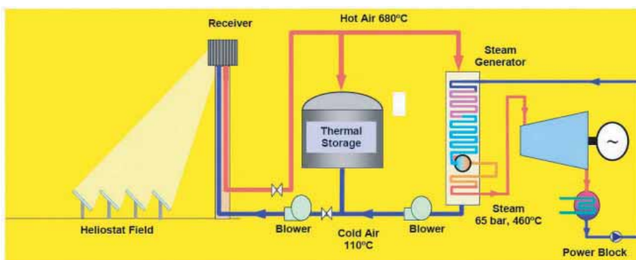
Solar Tower
