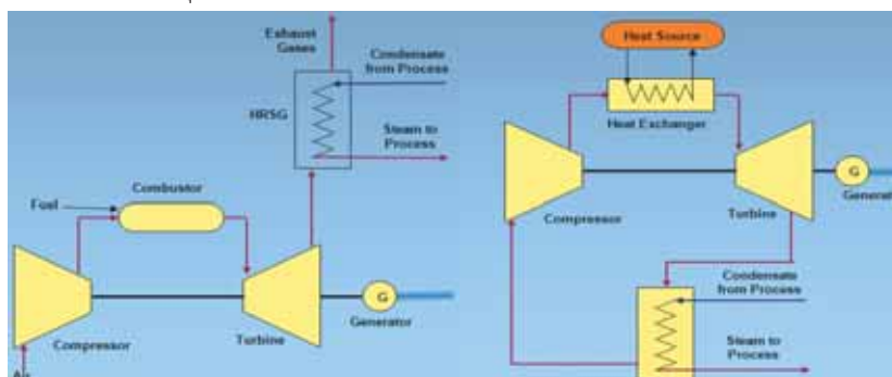
Open cycle gas turbine cogeneration System Closed Cycle Gas Turbine Cogeneration System
