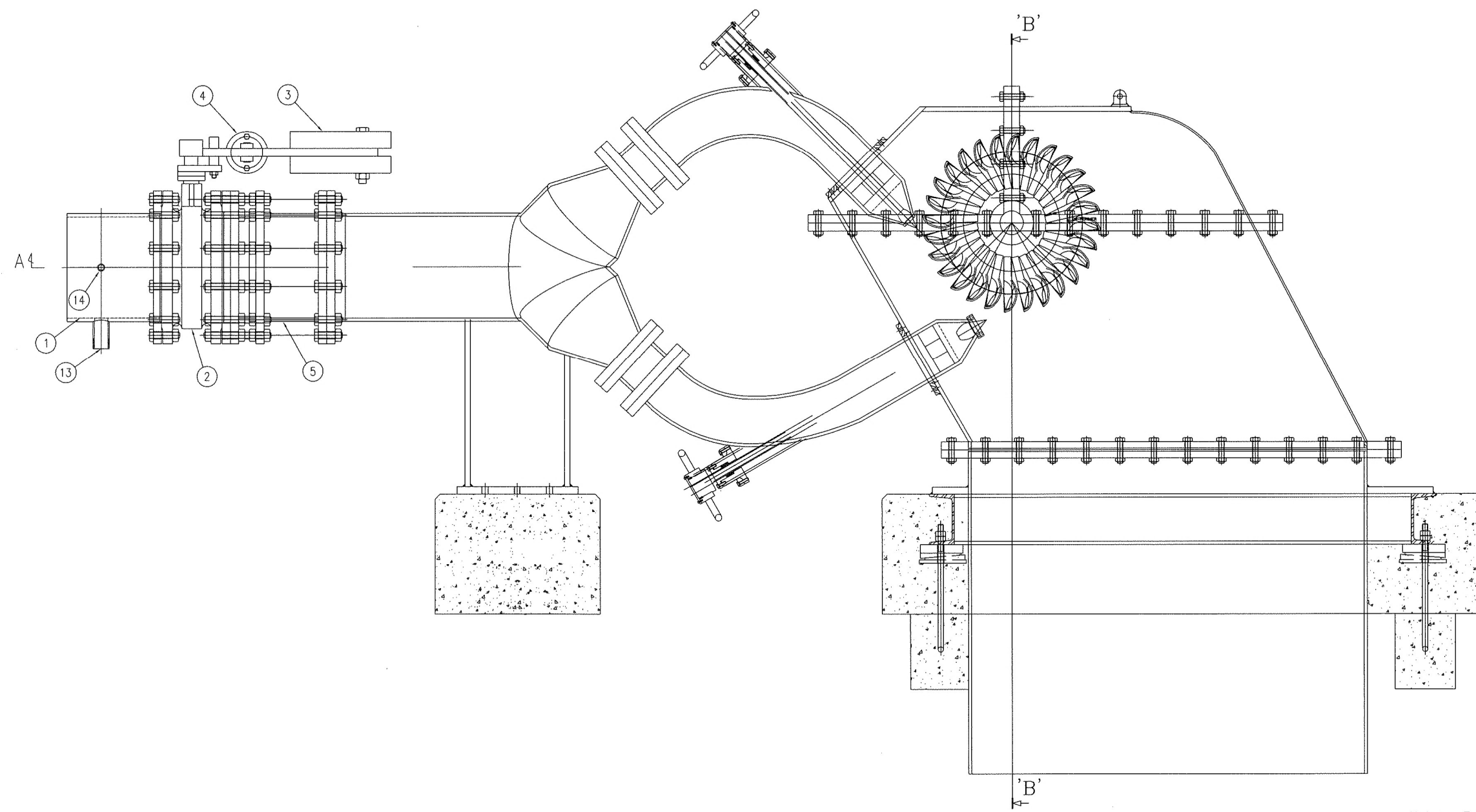
SECTION 'A'-'A'
