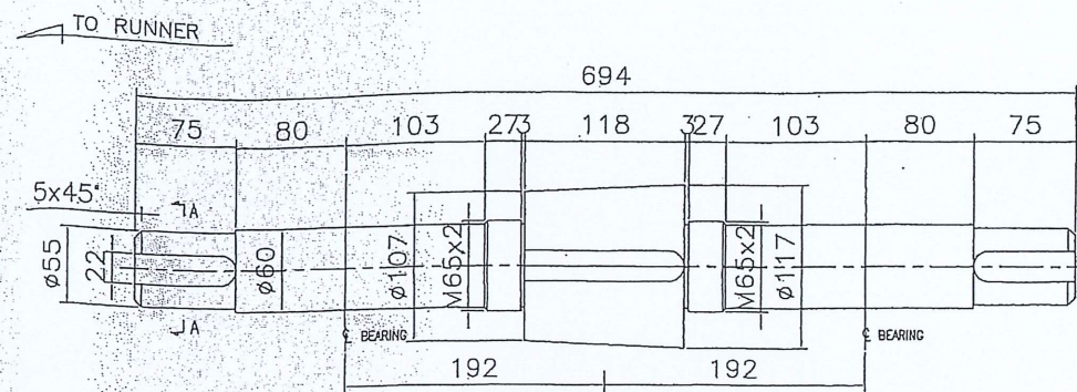
3 FLYWHEEL SHAFT SCALE 1:1.25
