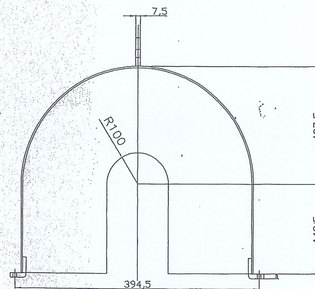
7 FLYWHEEL GUARD SCALE 1:1.25
