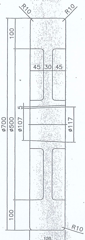
6 FLYWHEEL SCALE 1:1.25
