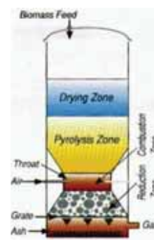
Downdraft Gasifier
