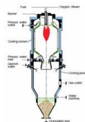
Entrained Bed Gasifier
