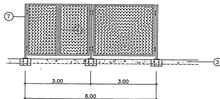
SECTION 0 - 0
