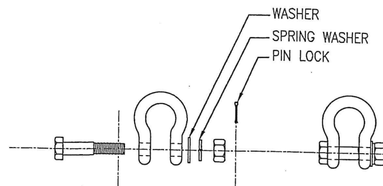
SHACKLE 5/8\"/>
