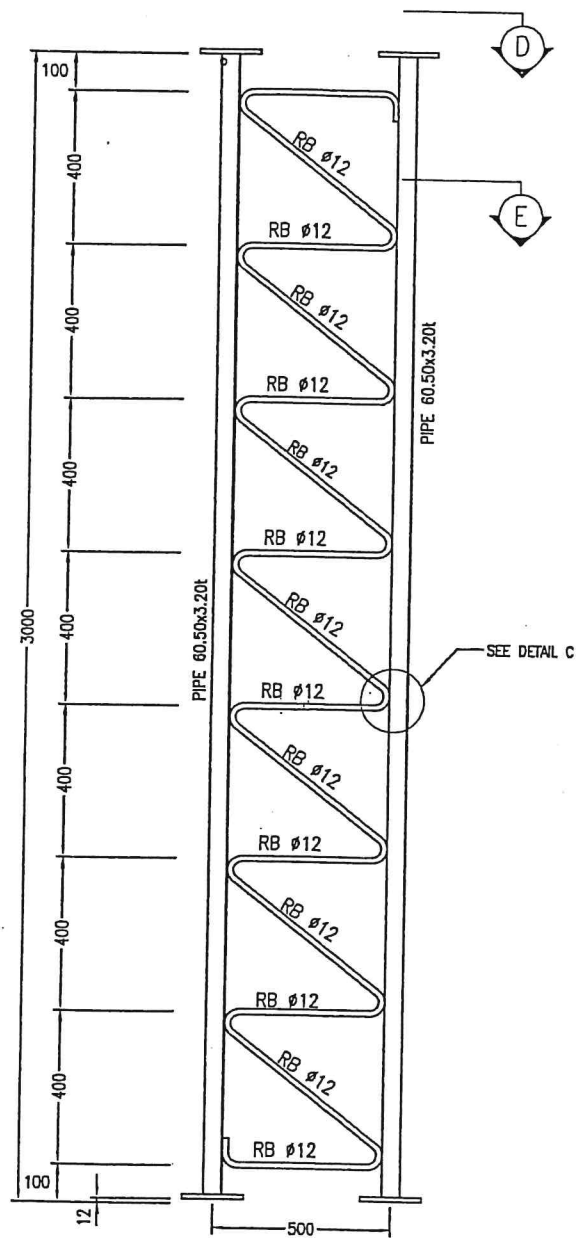
MAST SECTION 1:15
