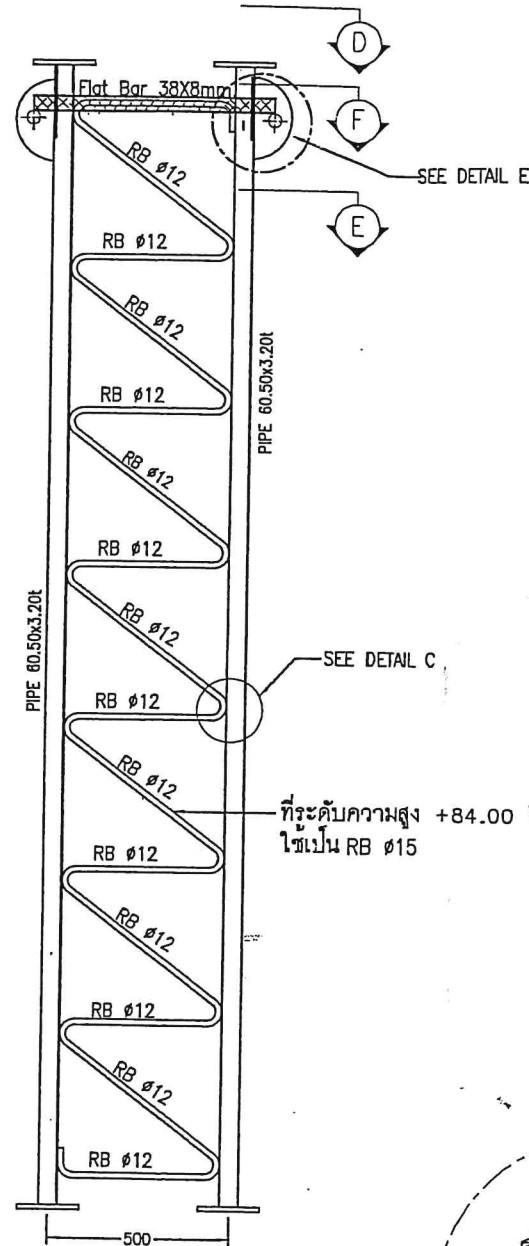
MAST TOP SECTION NTS.
