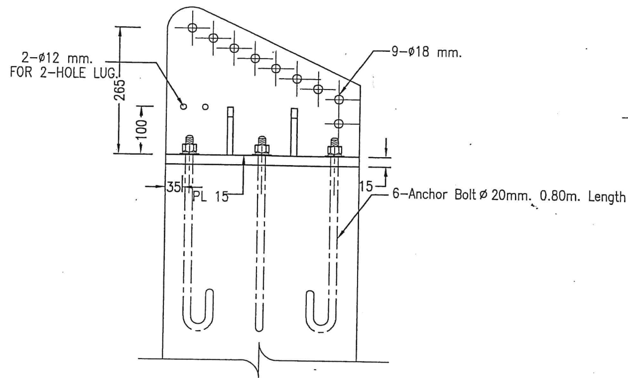
ANCHOR FRAME
