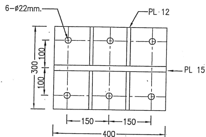
ANCHOR FRAME
